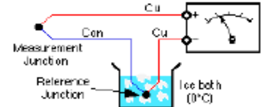
Traditional Thermocouple Measurement
