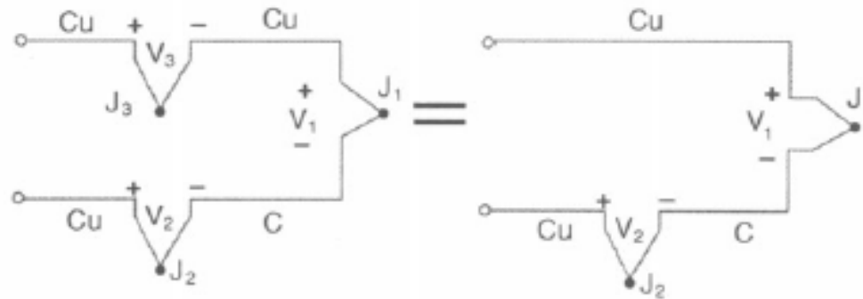
EQUIVALENT CIRCUITS
