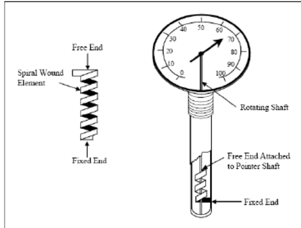
Figure 7-3. Bimetallic dial thermometer
